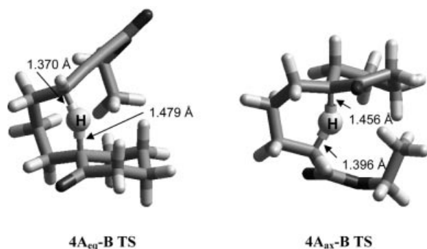
Figure 2. PM3 six-membered transition states for the 4A eq and 4A ax \rightarrow 4B hydrogen transfer.
