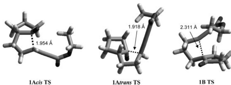
Figure 3. PM3 transition states for the 1A → 1A 1 and 1B → 1B 1 transformations.
