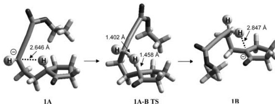
Figure 1. PM3 representations of the most stable conformers of anions 1A and 1B , and the transition state for hydrogen transfer ( 1A-B TS ) between them.
