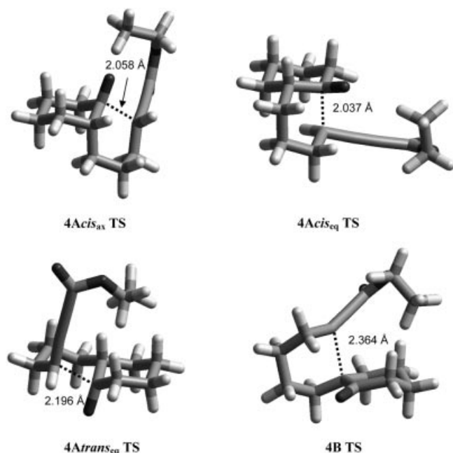
Figure 4. PM3 transition states for the 4A → 4A 1 and 4B → 4B 1 transformations.
