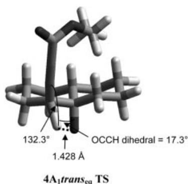
Figure 5. Transition state for direct hydrogen transfer in compound 4.
